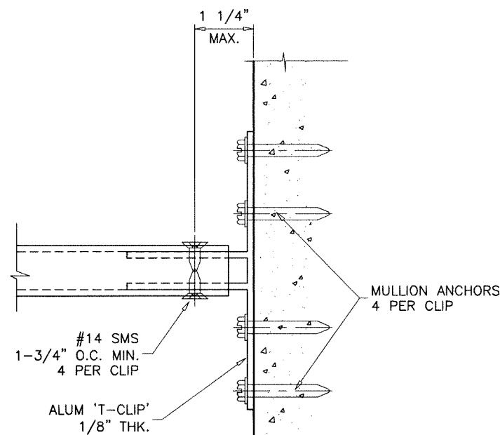
MULLION CONNECTION HORIZONTAL MULLION AT JAMBS
